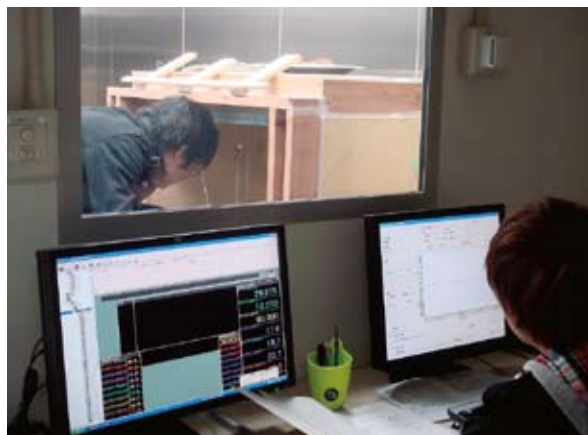
▲ 計測実験の様子：人工気候室での温熱環境実験 Measurements and experiments of the thermal environment
